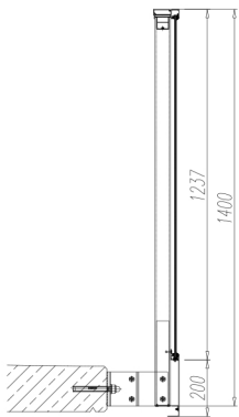
Balustrada FBD-1
